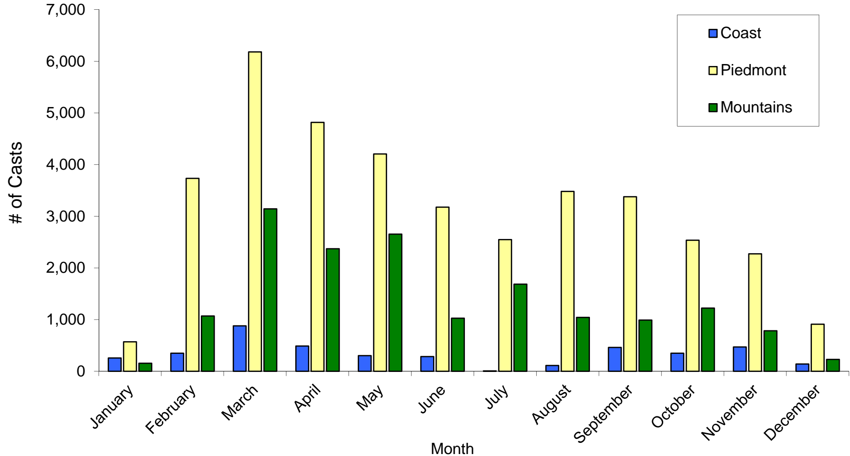
Figure 6. Number of casts reported by month and by region from the North Carolina RFTS, 1987 through February 2011.
