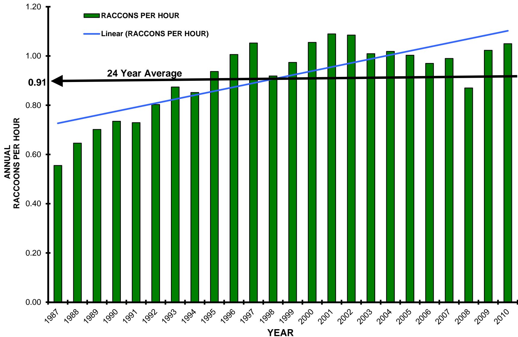
Figure 3. Statewide annual North Carolina RFTS results and 24-year average, 1987 through February 2011.
