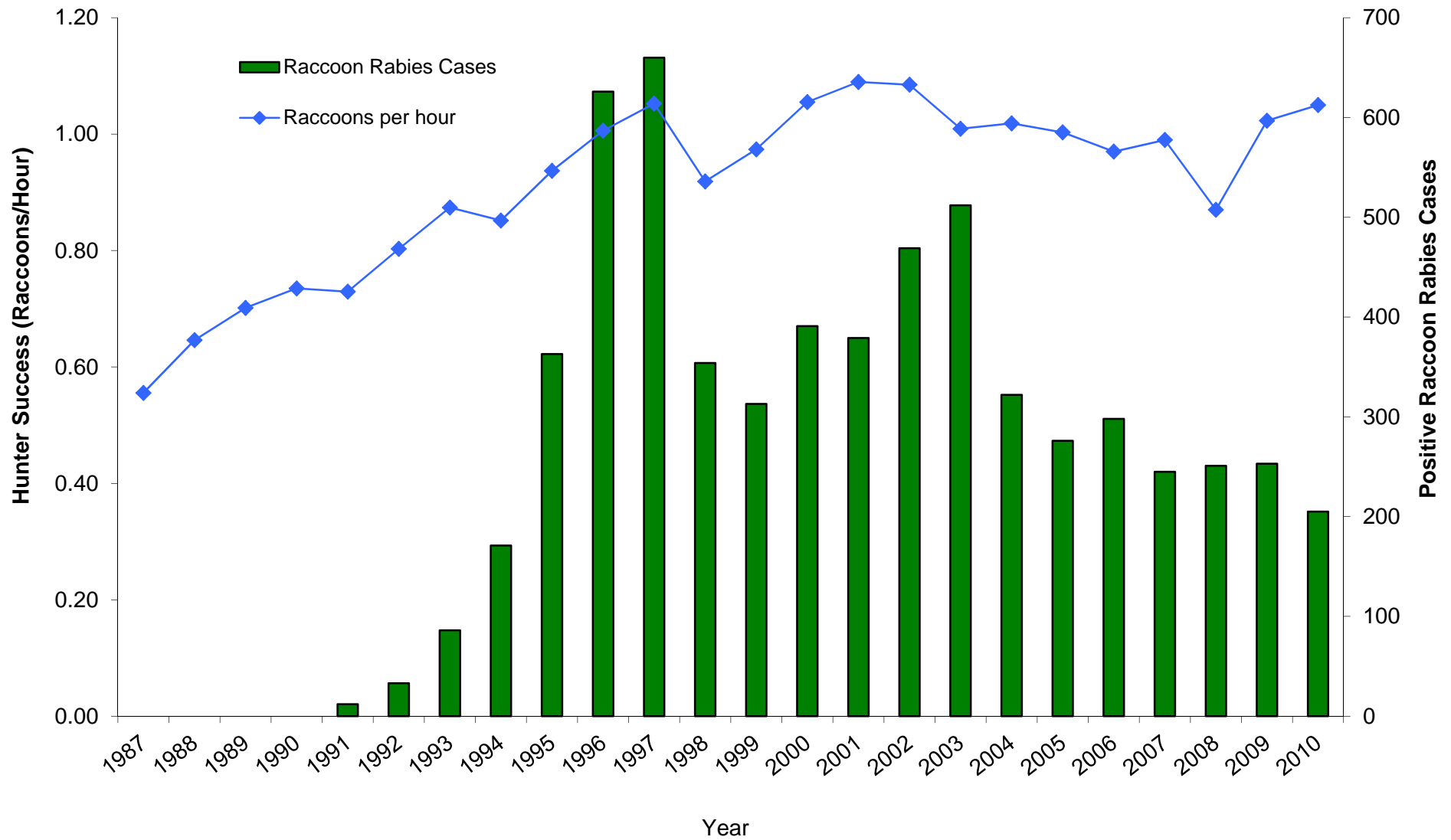
Figure 9. Annual statewide hunter success from the North Carolina RFTS and annual number of positive raccoon rabies cases.
