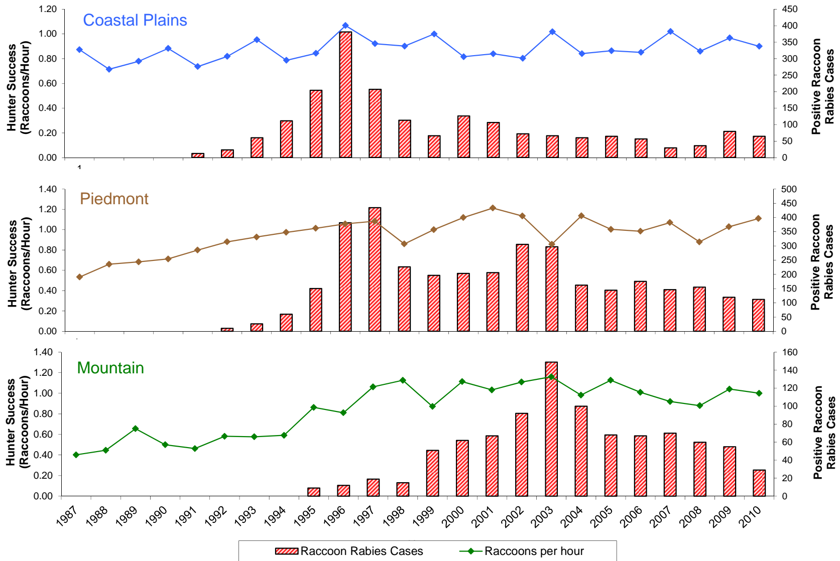
Figure 10. Annual regional hunter success from the North Carolina RFTS and annual number of positive raccoon rabies cases.
