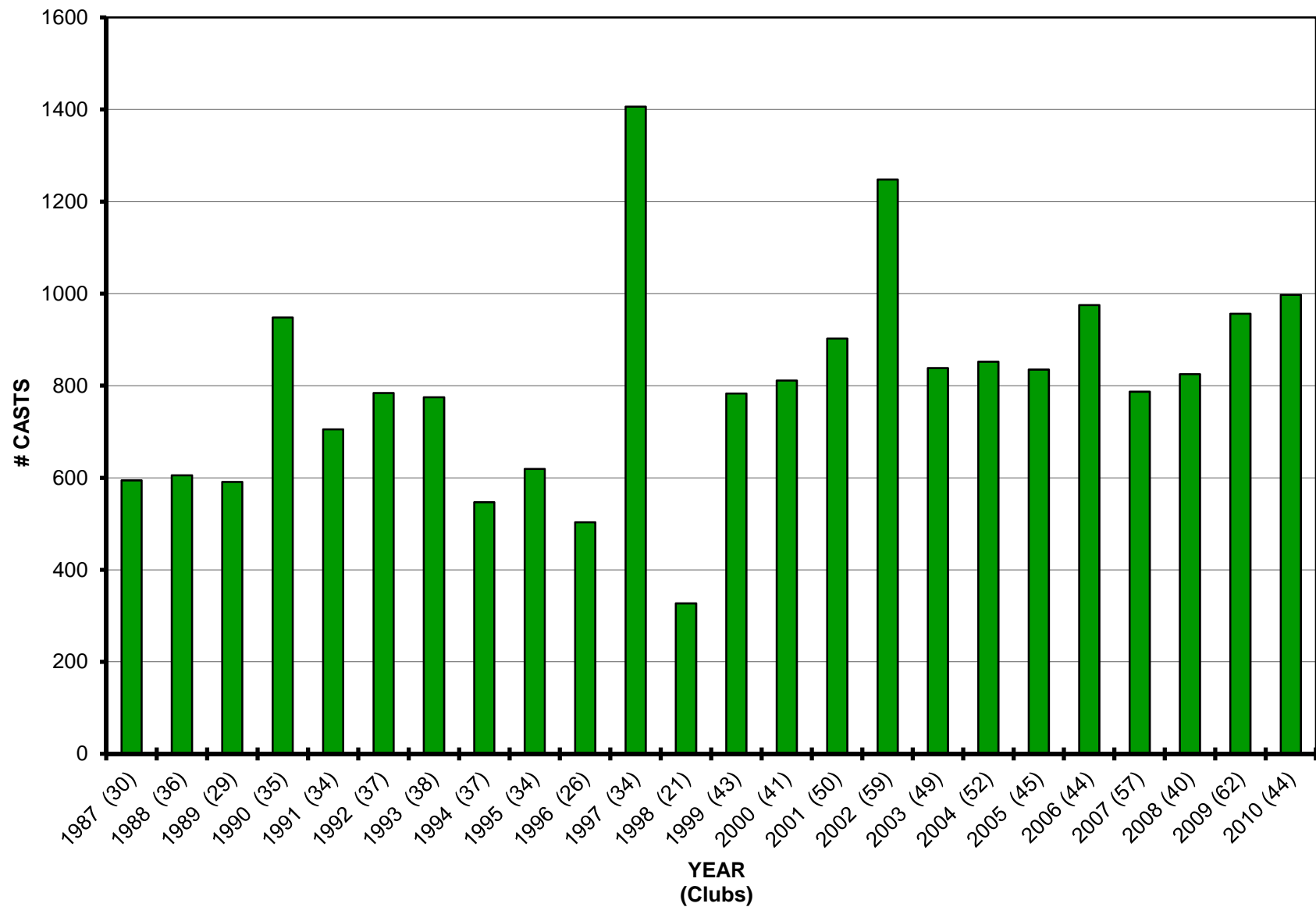
Figure 2. Annual number of casts and clubs participating in the North Carolina RFTS, 1987 through February 2011.
