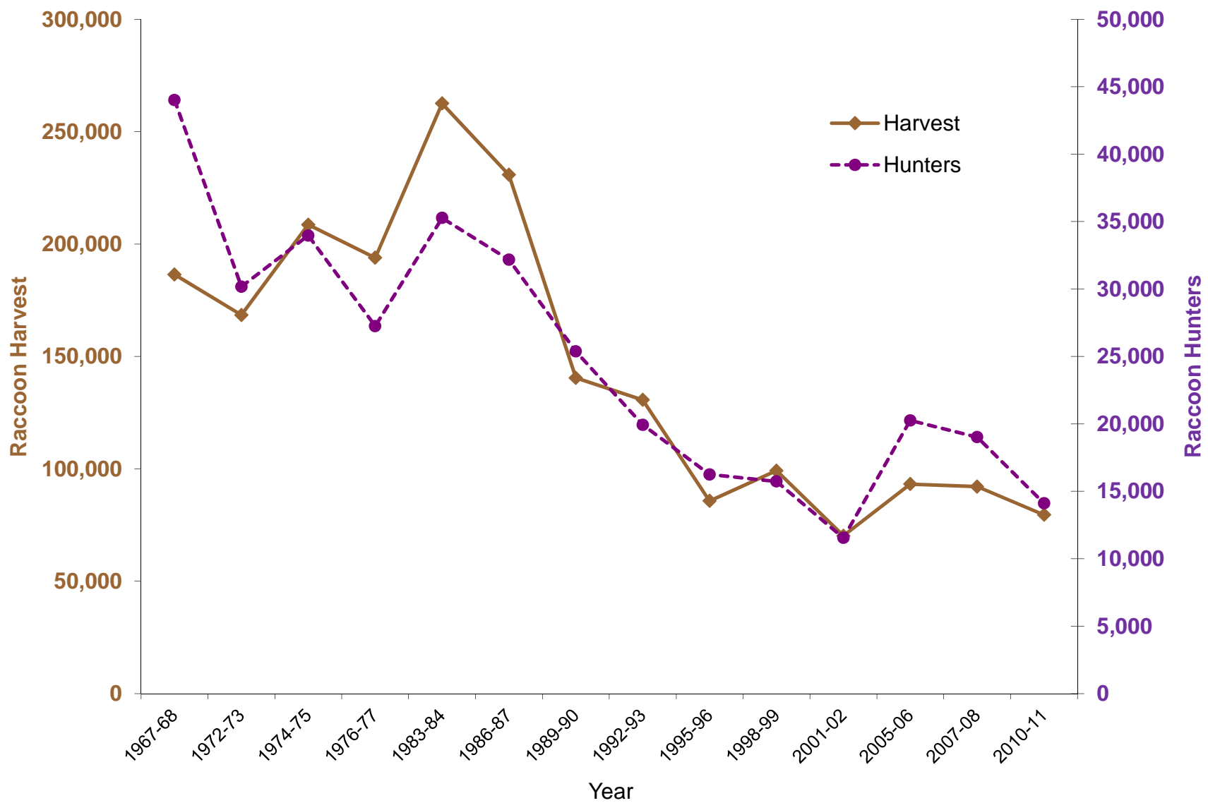
Figure 11. Number of raccoons harvested and number of raccoon hunters based on NCWRC Hunter Harvest Surveys, 1967 through 2011.
