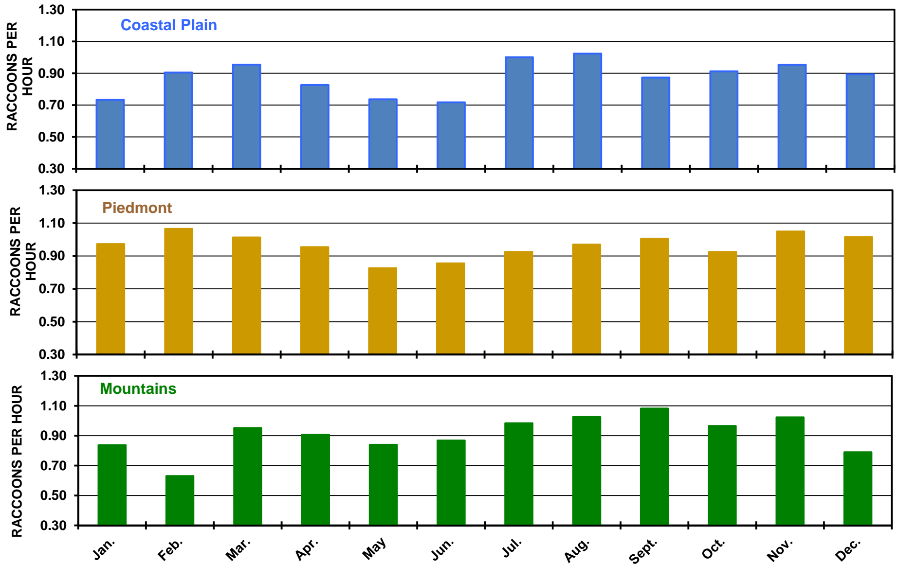
Figure 5. Regional hunter success reported by month from the North Carolina RFTS, 1987 through February 2011.
