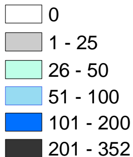
Figure 8. Number of positive terrestrial wildlife rabies cases reported by county, 1991-2010.
