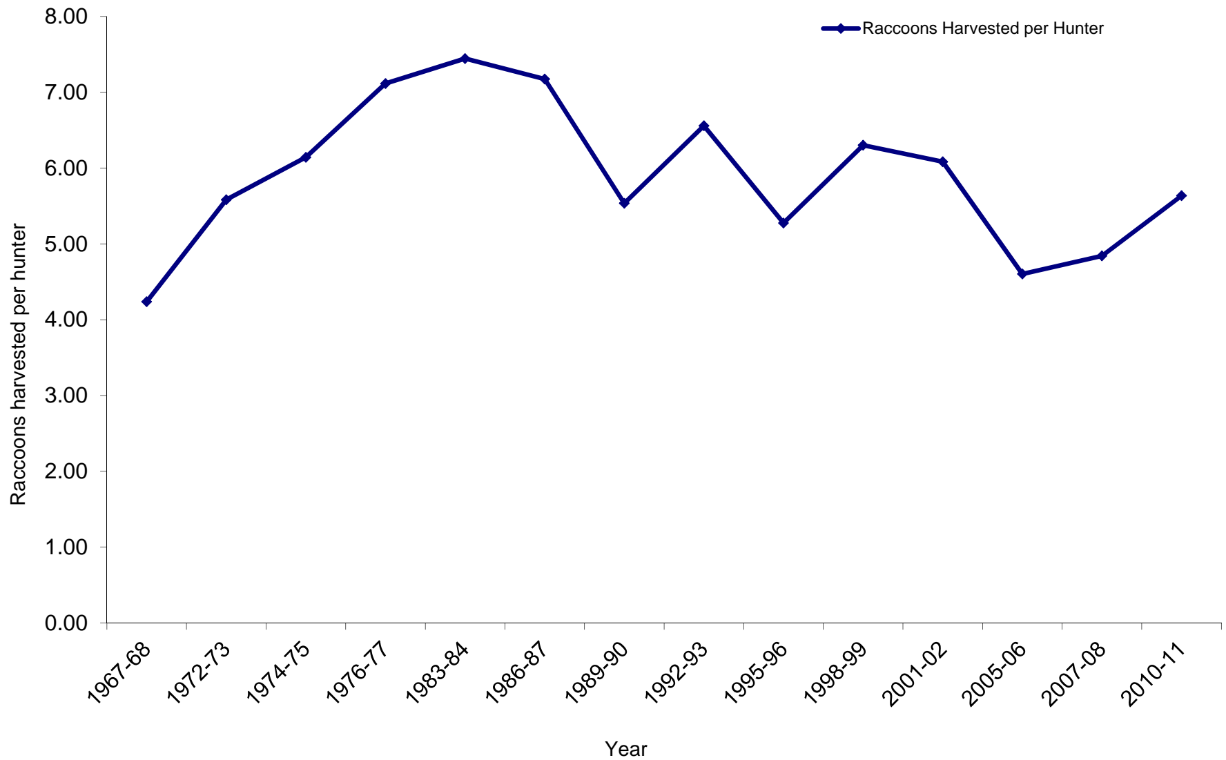
Figure 12. Number of raccoons harvested per hunter based on NCWRC Hunter Harvest Surveys, 1967 through 2011.
