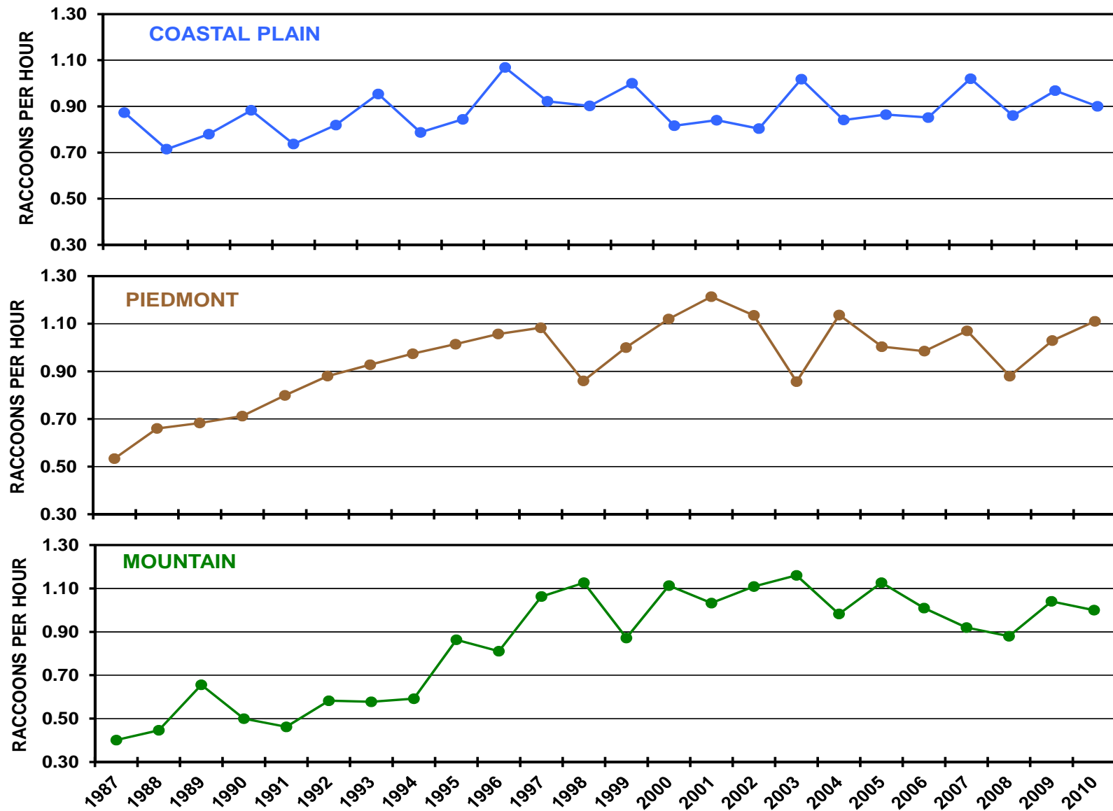
Figure 4. Regional annual hunter success from the North Carolina RFTS, 1987 through February 2011.
